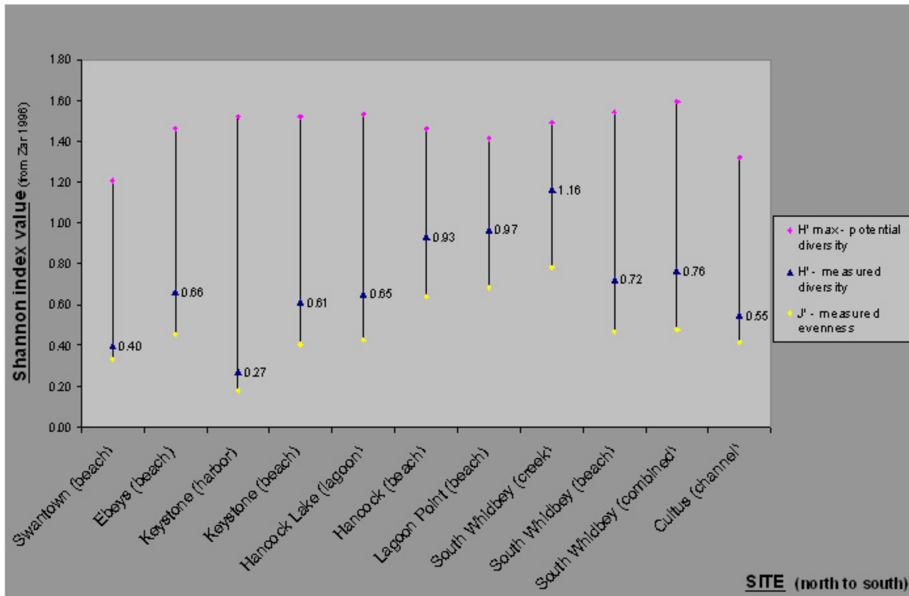
Figure 3 Species diversity and evenness for nearshore marine fish communities sampled with the large beach seine along the west coast of Whidbey Island.
